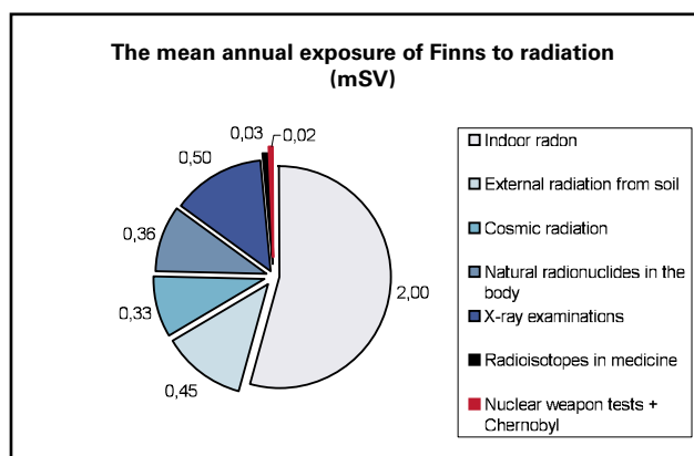
Fig. 1.3. A Finn gets annually about 3.7 millisievert dose from ionising radiation. The sources of radiation presented in this report cause in total about 0,7 % of the total dose (the red slice in the figure).
